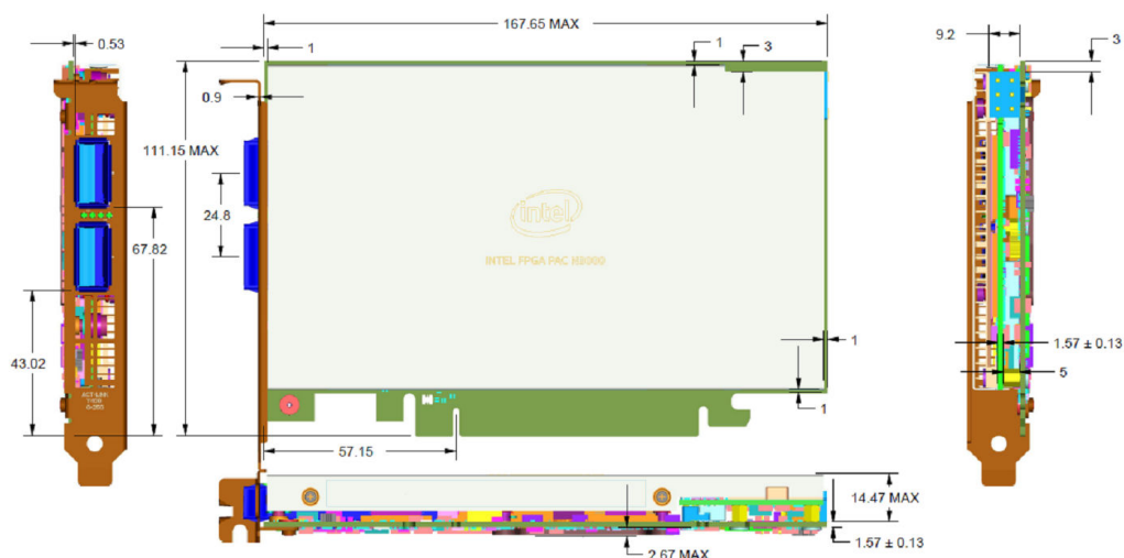
Figure 4. Intel FPGA PAC N3000 Dimensions
